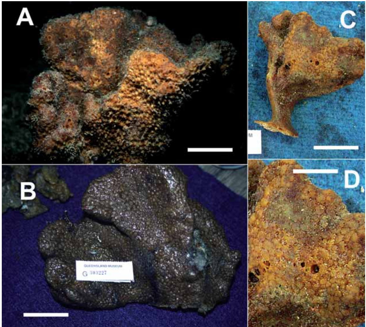
Fig. 4. Sollasella moretonensis n.sp.. A. Holotype QMG303227, alive (scale 6 cm), B. Holotype QMG303227, on deck after collection (scale 6 cm), C. Paratype QMG321402, on deck (scale 4 cm), D. Paratype QMG321402, close view of polygonal surface patterns around pores (scale 2 cm). (photos J.N.A. Hooper)
