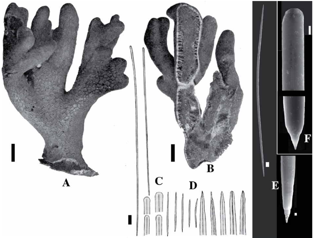
Fig. 1. Sollasella digitata Lendenfeld, 1888. A, habit of spirit specimen (scale 1 cm). B, BMNH lectotype (scale 1 cm). C, drawing of styles (scale 10 \mu m) and details of heads (same scale 1 \mu m). D, drawing of oxeas (scale 10 \mu m) and details of apices (scale 1 \mu m). E-F, SEM images of spicules (right scales 1 \mu m, left scale 10 \mu m). E, oxea and detail of apex. F, style. A-D, reproduced from Hallmann, 1914: pl. XV figs 1-2 and text-fig. 1. (the present figure entirely reproduced from van Soest, 2002).
