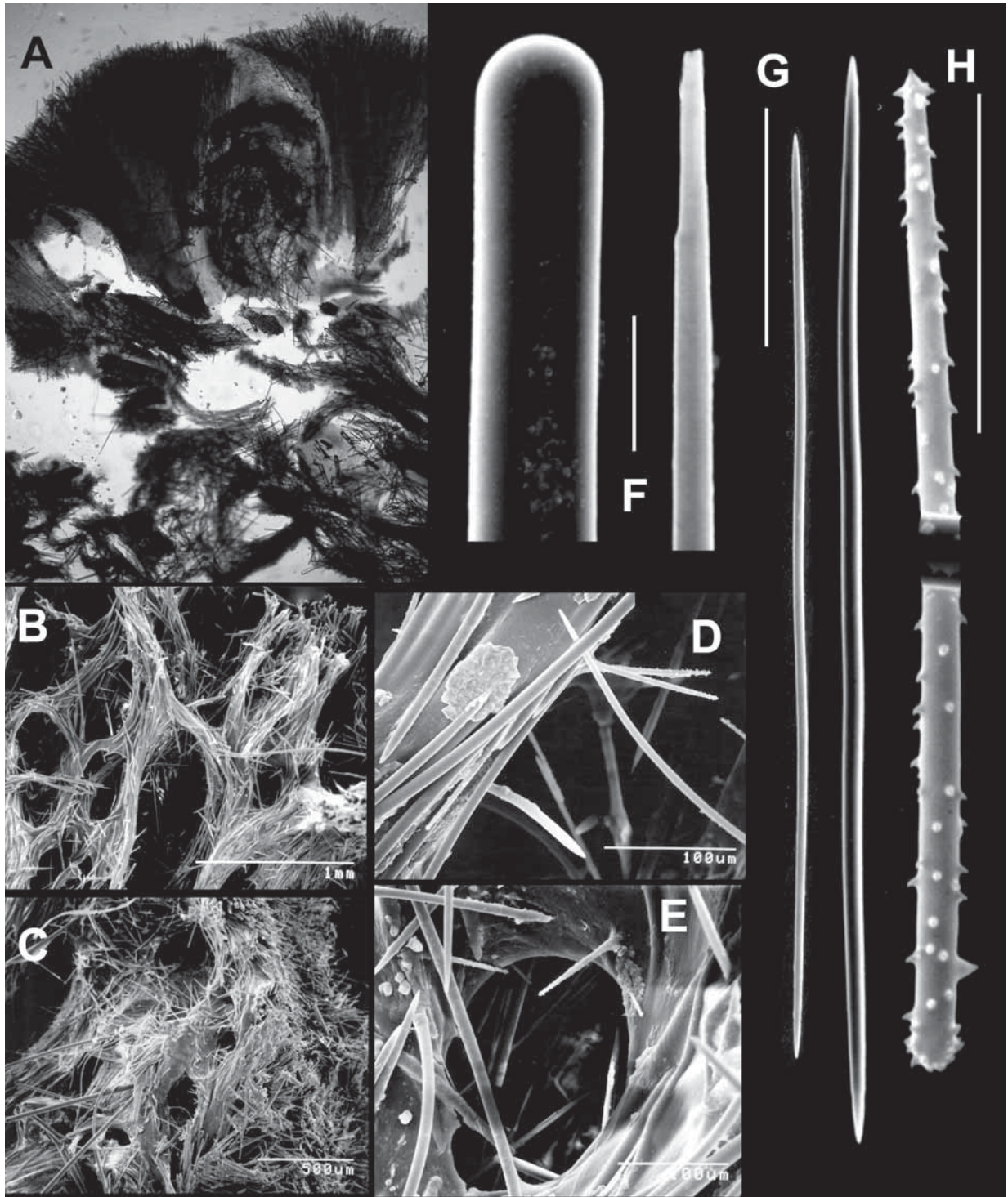
Fig 5. Sollasella moretonensis n.sp.. Holotype QMG303227. A. Light micrograph of skeleton (scale 1 cm), B. SEM of diffuse multi-compartmental axial skeleton (scale 1 mm), C. SEM of slightly radial peripheral skeleton (to the bottom left) (scale 500 \mu m), D. Acanthostyles echinating spongin fibres and associated bundles of choanosomal styles/ oxeas running parallel to fibres (scale 100 \mu m), E. Echinating acanthostyles protruding into fibre mesh (scale 100 \mu m), F. Base and point of long choanosomal style (scale 25 \mu m), G. Ectosomal oxeas (scale 200 \mu m), H. Echinating acanthostyle (scale 50 \mu m).
